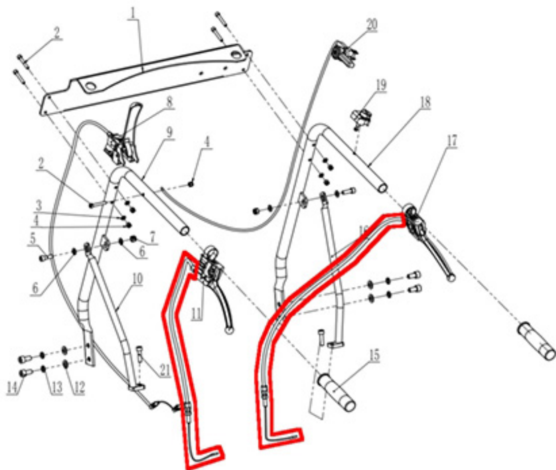
Dumper Thomas SF 2610A
